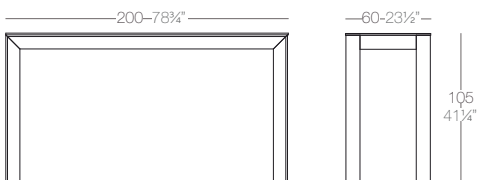
FRAME Mesa Aluminio 200 x 60 x 105 cm FRAME Table Aluminio Base 78 3/4" x 23 1/2" x 41 1/4" ref: 54152
