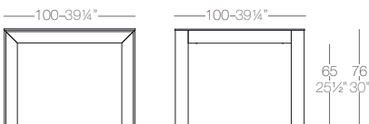
FRAME Mesa Aluminio 100 x 100 x 76 cm FRAME Table Base Aluminio 39 1/4" x 39 1/4" x 30" ref: 54117
