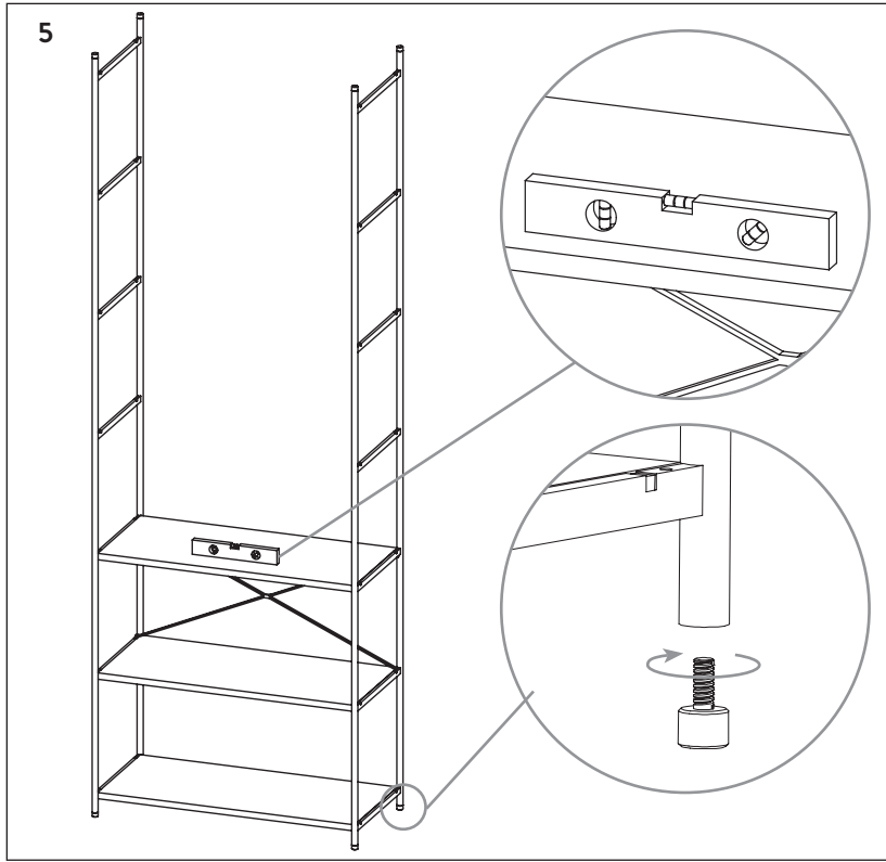
5. Use a spirit level and adjust the four adjustment screws. Then tighten the four screws for the cross.
