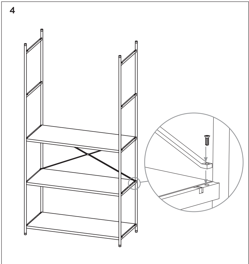
4. Attach the cross just above the second shelf and screw all four screws lightly. Do not tighten the screws yet.
