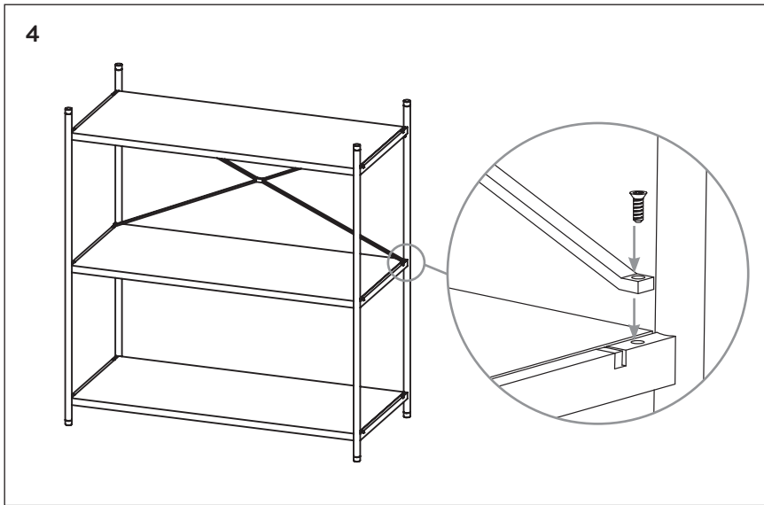
4. Attach the cross above the second shelf and screw all four screws lightly. Do not tighten the screws yet.
