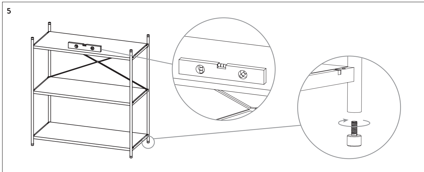
5. Use a spirit level and adjust the four adjustment feet. Then tighten the four screws for the cross.
