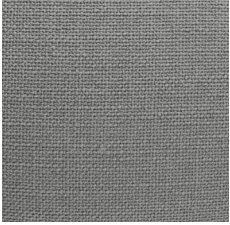
Pilling-resistant fabric
